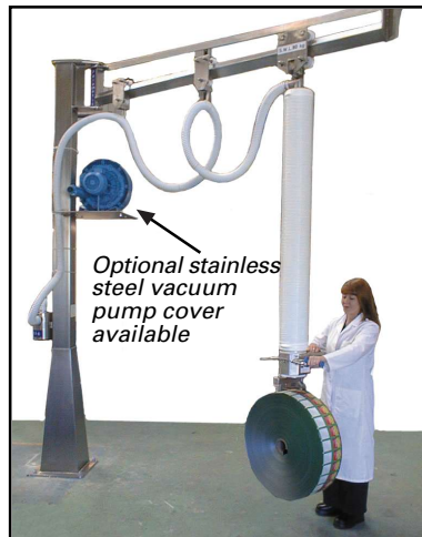
Vacuum Tube Lifter handling 50kg (110lbs) reels supported from a stainless steel floor mounted support column with 3m (10') PalTrac swing jib.
