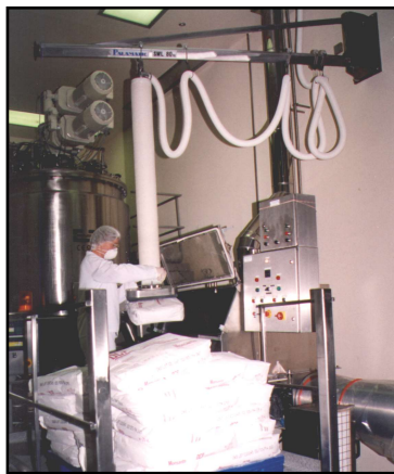
Wall mounted swing jib arrangement and vacuum tube lifter handling sacks from a pallet into a sack tip booth.
