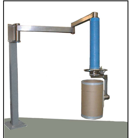
Vacuum Tube Lifter handling 50kg (110lbs) fibre drums supported from a floor mounted support column with 3m (10') articulated arm manufactured in 304 stainless steel.
