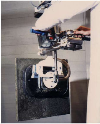
REF NO: REF-VG-007 WEIGHT: 35kg FEATURES: Vacuum grip 90° powered rotation
