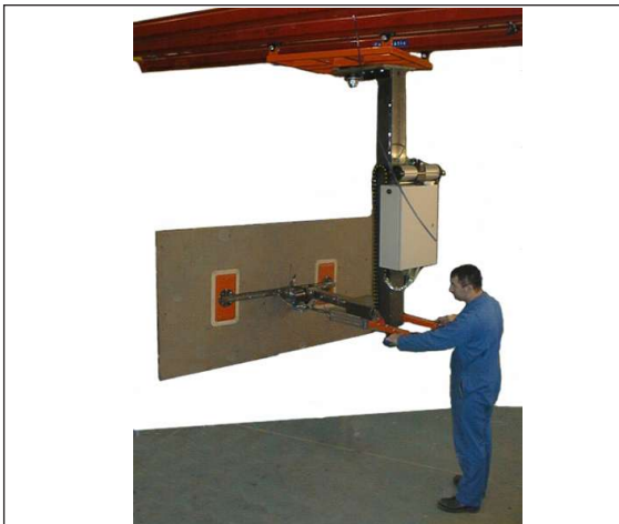
REF NO: PIL-VG-001 FEATURES: Pillar Lift handling 120kg wooden boards and turning 90° to load laser machines
