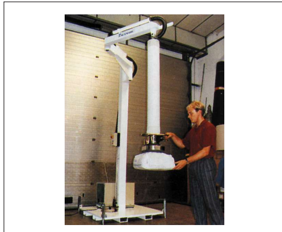
REF NO: MO-VG-004 FEATURES: Mobile sack lifter. Can be transported by fork lift truck or pallet truck. SWL 60kg
