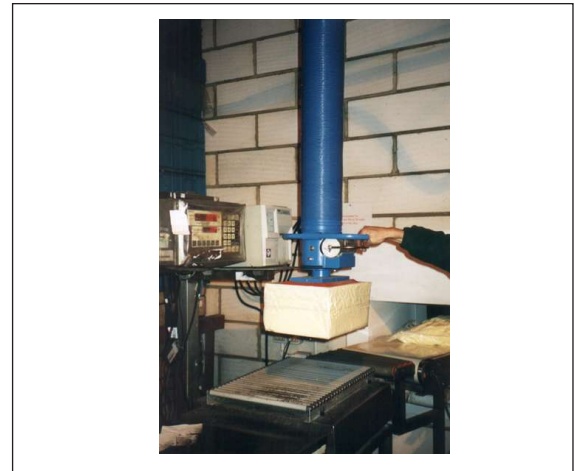
REF NO: F-VG-004 WEIGHT: 6kg FEATURES: Vacuum grip with food grade seal handling 30kg cheese blocks
